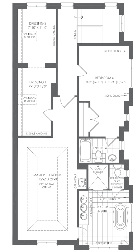
THIRD FLOOR ELEV. A
