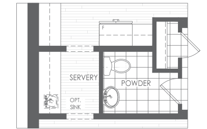
OPTIONAL SERVERY GROUND FLOOR ELEV. A & B
